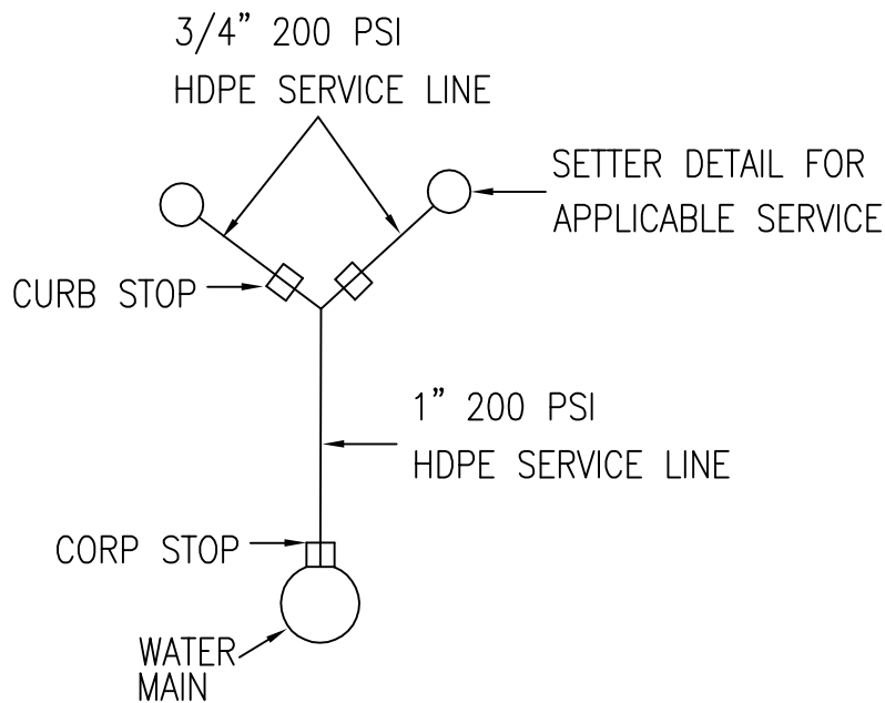
DUAL SERVICE WITH ONE TAP OFF MAIN
